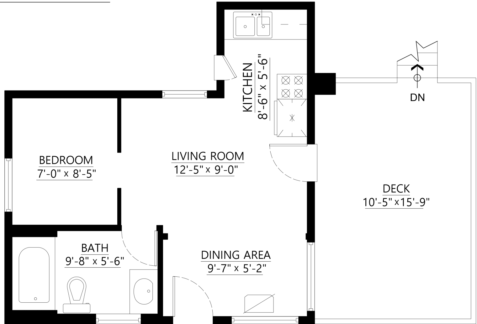
Rockaway Cottage Floor Plan Floor Area: 359 sq.ft.
