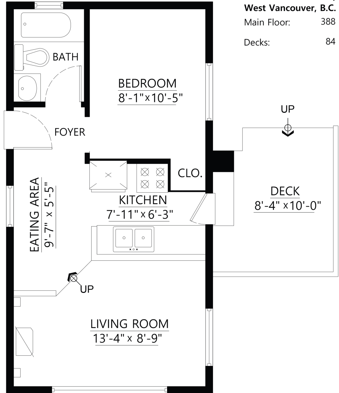
Maples Cottage Floor Plan Floor Area: 388 sq.ft.
