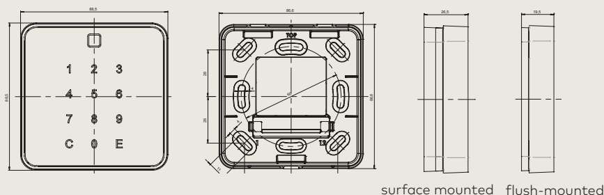
dormakaba registration unit 90 02 Front and rear panel
