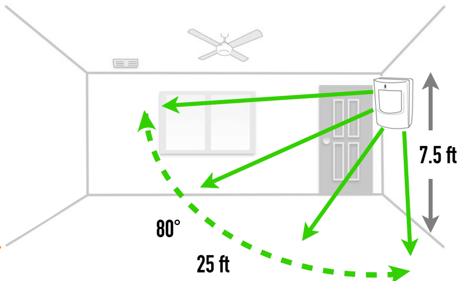
Wall install
