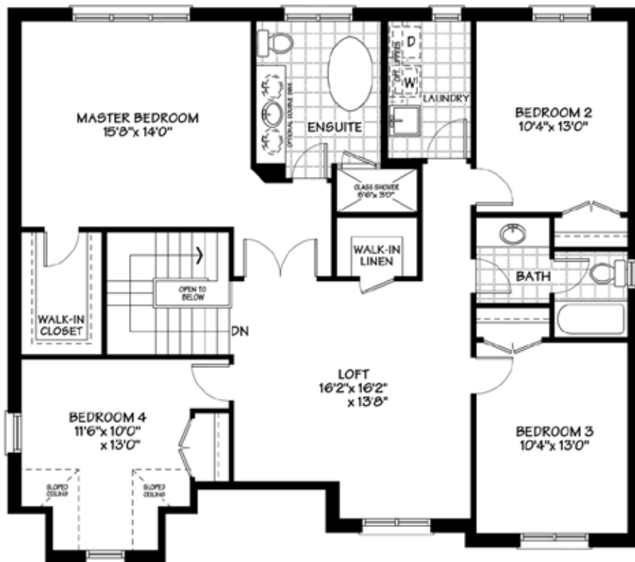
ALTERNATE SECOND FLOOR PLAN ELEV - A
