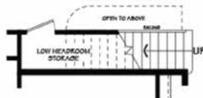
MAIN FLOOR LOFT CONDITION
