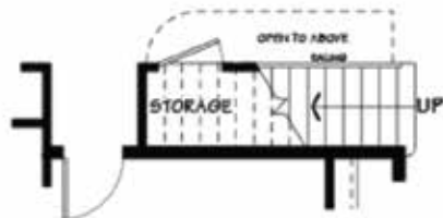
MAIN FLOOR LOFT CONDITION OPTIONAL 3-BEDROOM
