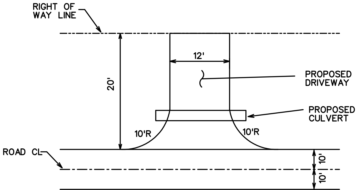
TYPICAL DRIVEWAY PLAN N.T.S.
