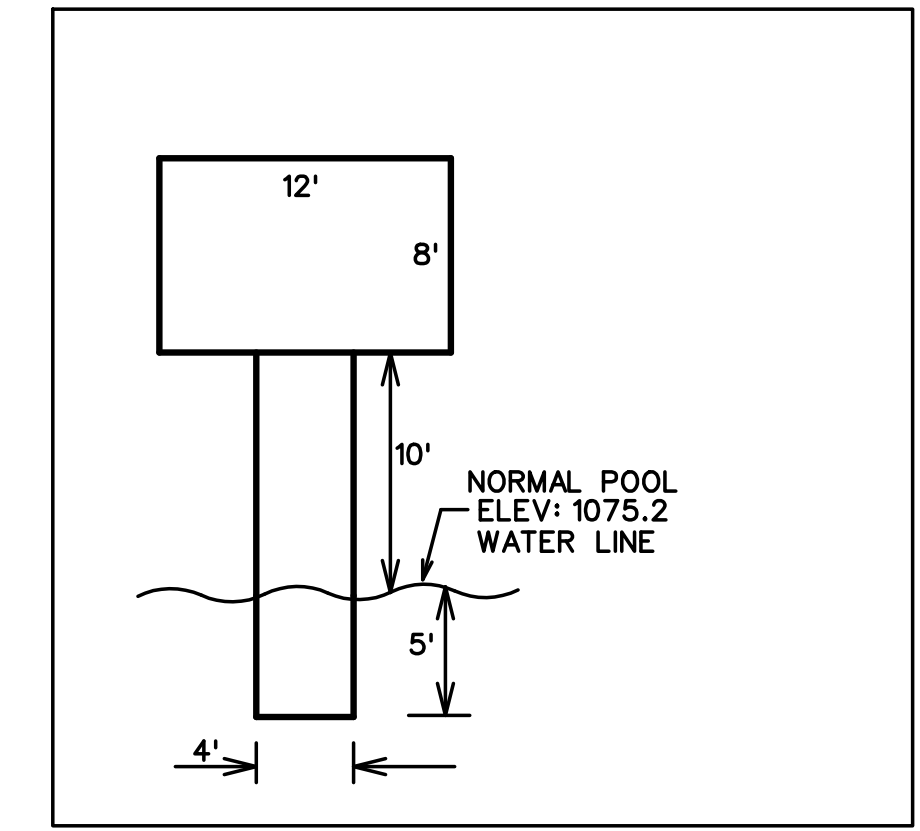
PROPOSED DOCK (TYP.) N.T.S.
